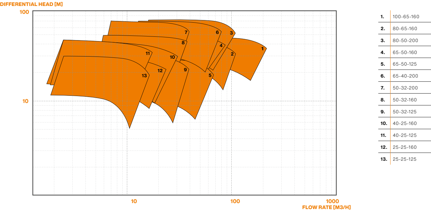
PERFORMANCE RANGE CHARTS 2.950 MIN -1 (50 HZ)
