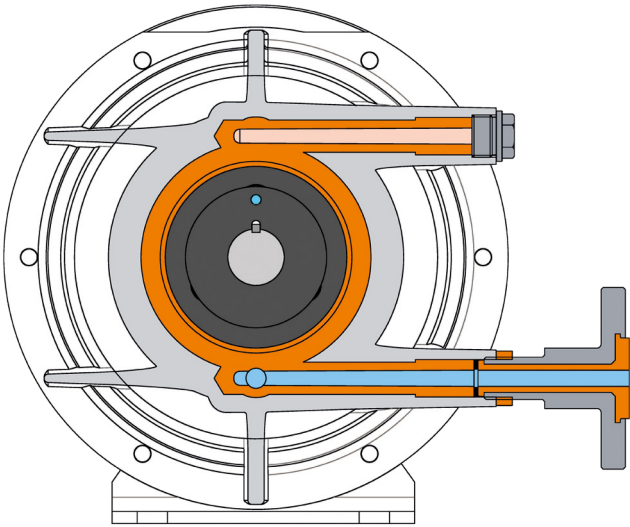
Flushing connection for plain bearing lubrication from an external source
