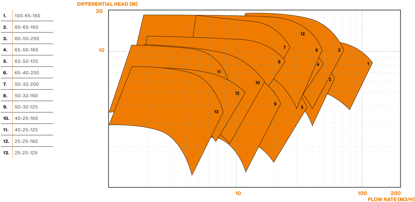
PERFORMANCE RANGE CHARTS 1.450 MIN -1 (50 HZ)
