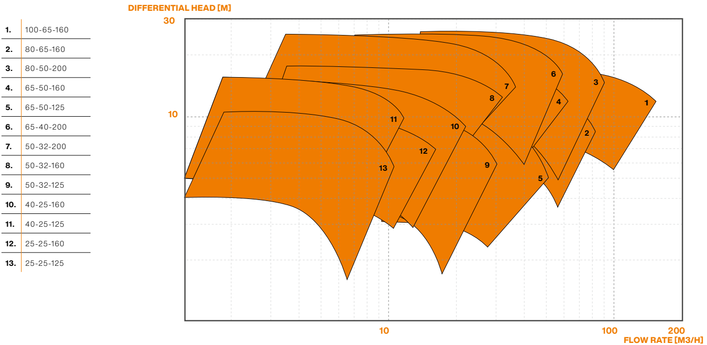
PERFORMANCE RANGE CHARTS 1.750 MIN -1 (60 HZ)
