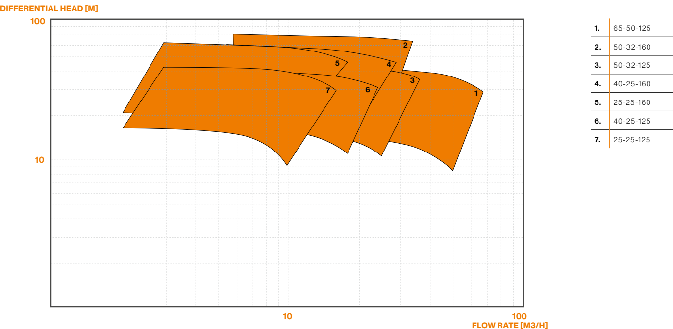
PERFORMANCE RANGE CHARTS 3.550 MIN -1 (60 HZ)
